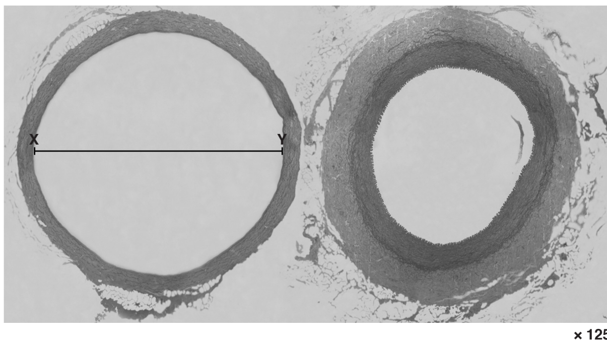
vein
